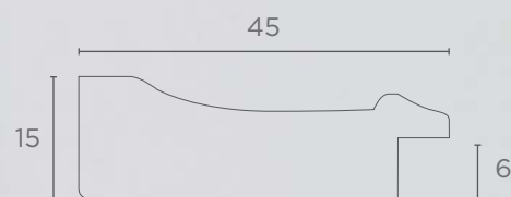
PA-45
