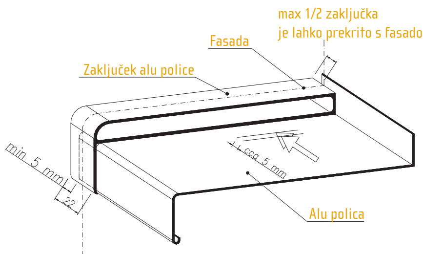
Detajl alu police
