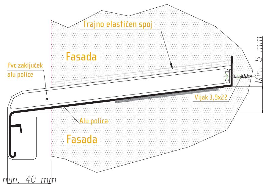
Prerez police
